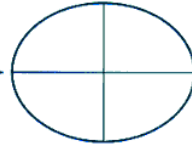
Ellipsoid
