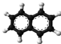
Naftalin: C_{10}H_8
