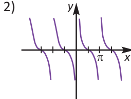
b) y = \cot \left(x + \frac{\pi}{2}\right)
